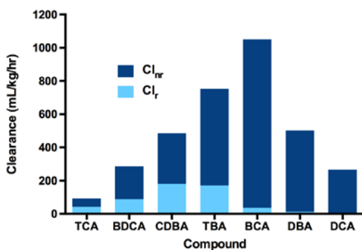
Figure 3-5. Comparison of renal (Cl r ) and nonrenal (Cl nr ) clearance of an equimolar i.v. dose (500 \mu mol/kg) of haloacetic acids in male rats
